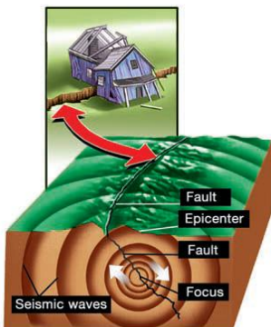
Figure 12.2: The focus, epicenter, and seismic waves of an earthquake occurring at an active fault.
