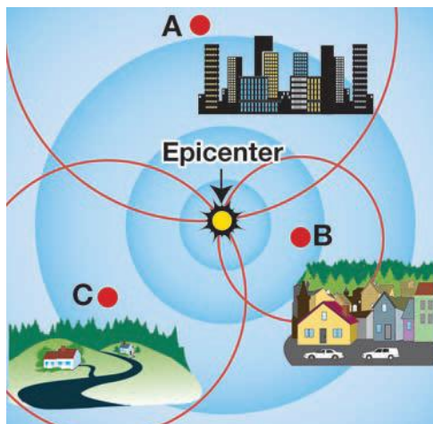
Figure 12.8: An epicenter is located using data from three seismic stations.
